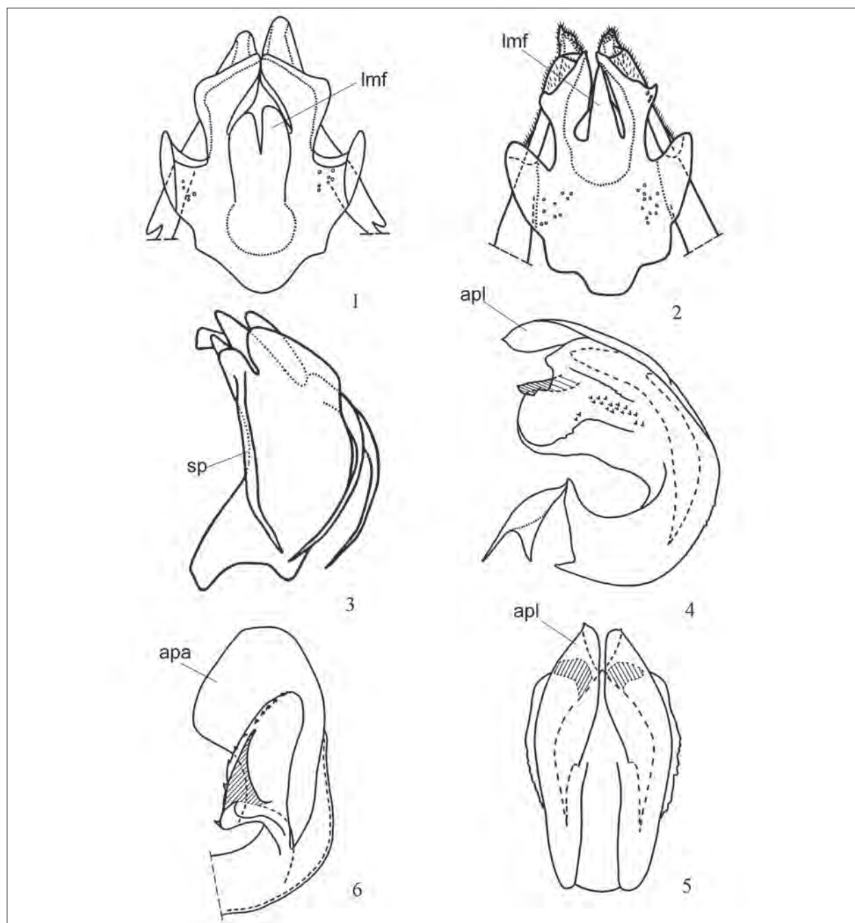
Plate 10. 1, Latematium latifrons (Fieber), posterior connective lamina of gonapophyses IX, dorsal view (after Gnezdilov, 2002c); 2, Pamphylum cypriacum (Dlabola), posterior connective lamina of gonapophyses IX, dorsal view (after Gnezdilov & Wilson, 2007a); 3, Phasmena breviuscula Emeljanov, penis, lateral view (after Emeljanov, 1978, modified); 4, Kervillea coronata (Logvinenko), penis, lateral view (after Gnezdilov, 2002b); 5, same, ventral view (after Gnezdilov, 2002b); 6, Tshurtshurnella uvarovi Gnezdilov, penis, lateral view (after Gnezdilov, 2002d).
